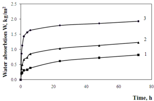
Fig. 2. Water absorption rates from water surface of ETICS samples: 1 – with mineral render; 2 – with acrylic render; 3 – with mineral render (double glass mesh)
