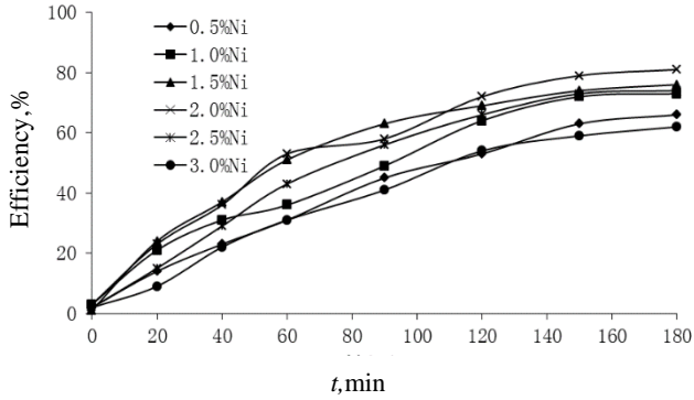
Fig. 5. \text{TiO}_2 degradation rates for different amounts of nickel doping
