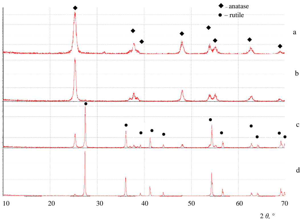
Fig. 1. XRD spectra for pure \text{TiO}_2 for different calcination temperatures: a–400 °C; b–500 °C; c–600 °C; d–700 °C
