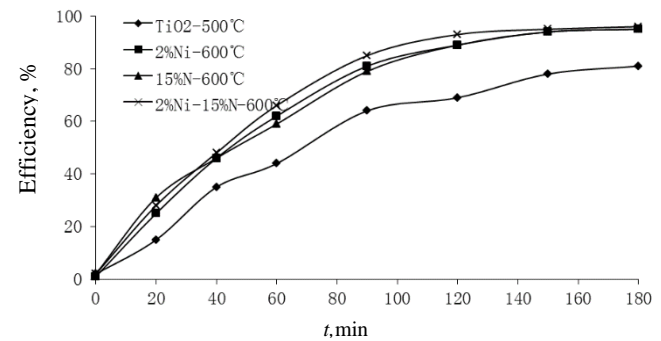
Fig. 8. Ultrasonic photocatalytic degradation effects of different catalysts
