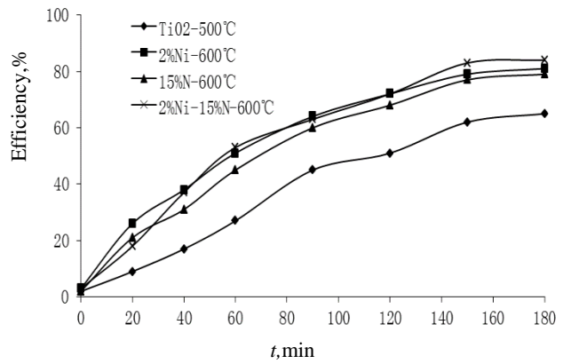
Fig. 7. Photocatalytic degradation effects of different catalysts
