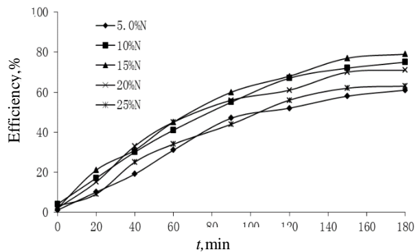
Fig. 6. \text{TiO}_2 degradation rates for different amounts of nitrogen doping
