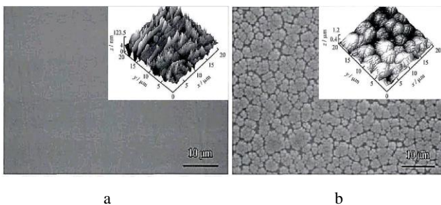
Fig. 2. SEM and AFM morphologies of: a–the uncoated 45 steel; b–the Ni-B coated 45 steel [37]
