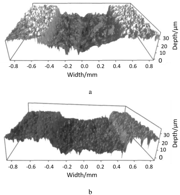
Fig. 1. 3D-morphology of wear scars: a – in distilled water; b – in sea water [18]
