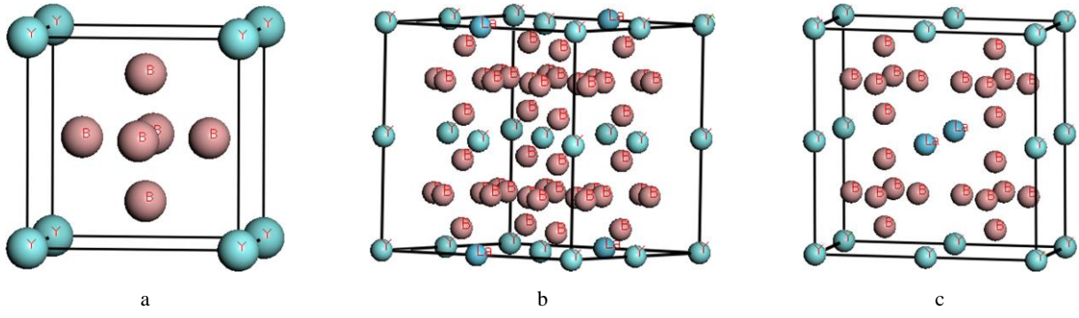
Fig. 1. Supercell structure: a – \text{YB}_6 ; b – \text{La}_{0.125}\text{Y}_{0.875}\text{B}_6 ; c – \text{La}_{0.25}\text{Y}_{0.75}\text{B}_6
