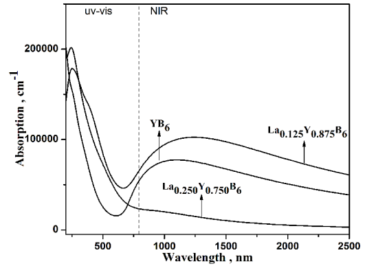
Fig. 6. The absorption spectra of \text{YB}_6 , \text{La}_{0.125}\text{Y}_{0.875}\text{B}_6 and \text{La}_{0.25}\text{Y}_{0.75}\text{B}_6
