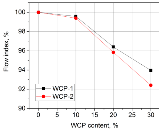
Fig. 6. Flow index versus WCP content for specimens
