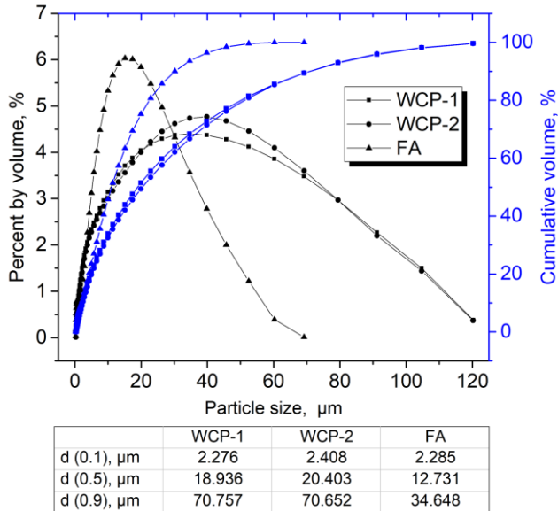
Fig. 1. PSD of WCP and FA by laser diffraction
