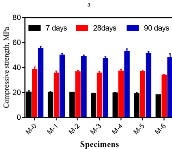
Fig. 7. Strength versus WCP content for specimens at 7, 28, and 90 days: a – flexural strength; b – compressive strength
