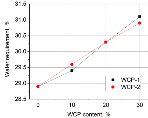
Fig. 4. Water requirement versus WCP content for specimens
