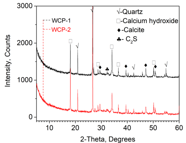
Fig. 2. XRD pattern of WCP-1 and WCP-2
