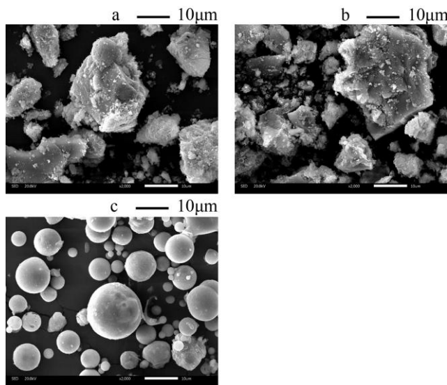
Fig. 3. SEM micrographs of WCP and FA: a–WCP-1; b–WCP-2; c–FA
