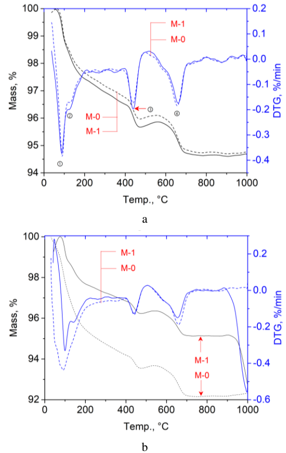
Fig. 9. DTG-TG curves of specimens: a–7 days; b–90 days
