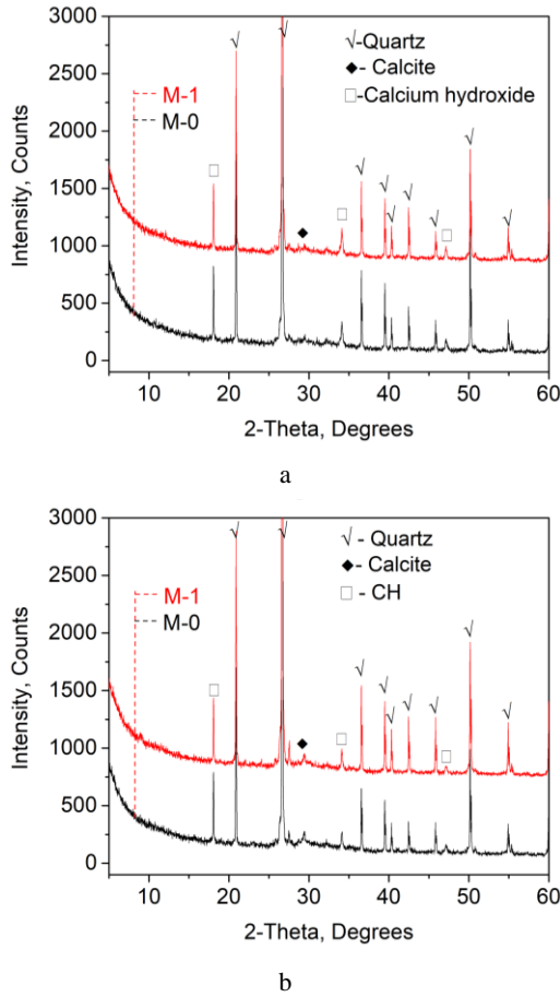
Fig. 8. XRD patterns of specimens: a–7 days; b–90 days
