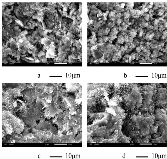
Fig. 10. SEM micrographs of specimens: a–fly ash mortar without WCP-1 at 7 days; b–fly ash mortar with WCP-1 at 7 days; c–fly ash mortar without WCP-1 at 90 days; d–fly ash mortar with WCP-1 at 90 days
