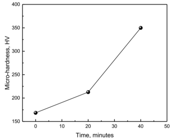
Fig. 4. Vickers hardness test of Al
