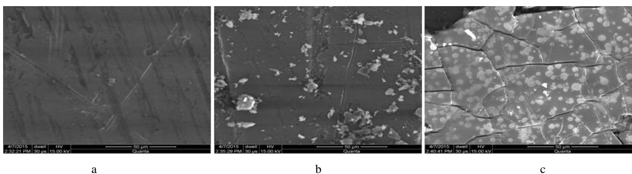
Fig. 2. SEM micrographs of Al target: a – unexposed Al at 1000\times ; b – 20 minutes exposed at 1000\times ; c – 40 minutes exposed at 1000\times
