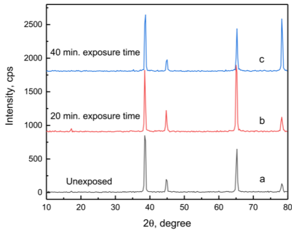
Fig. 3. The XRD patterns of the Al sample, a – unexposed Al sample; b – 20 minutes irradiated sample; c – 40 minutes irradiated sample
