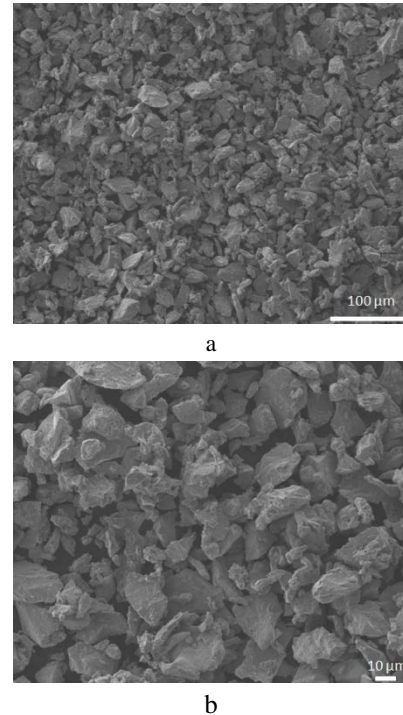
Fig. 1. SEM morphology of the original Cr 3 C 2 powder: a – low magnification; b – high magnification
