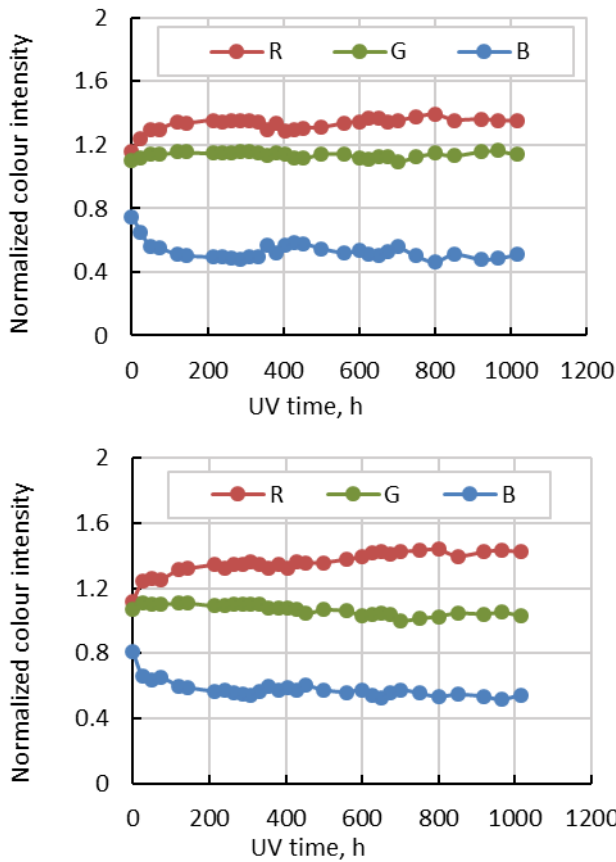
Fig. 8. R, G, B channels values normalized to Mean value for neat epoxy samples (top) and filled samples in colourless phase (bottom) during UV exposure
