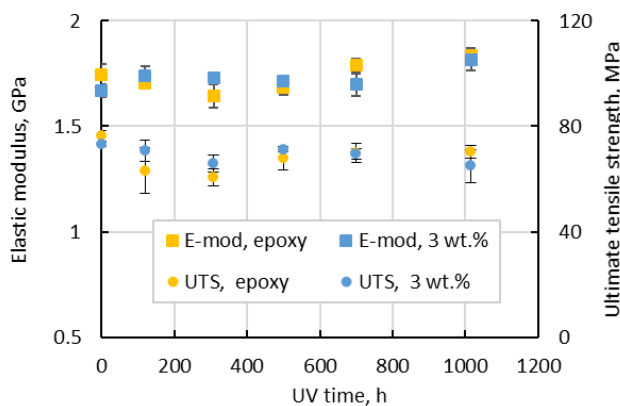
Fig. 15. Elastic modulus (■) and ultimate tensile strength (●) dependence on UV exposure time for neat epoxy (yellow) and filled with 3 wt.% (blue) samples
