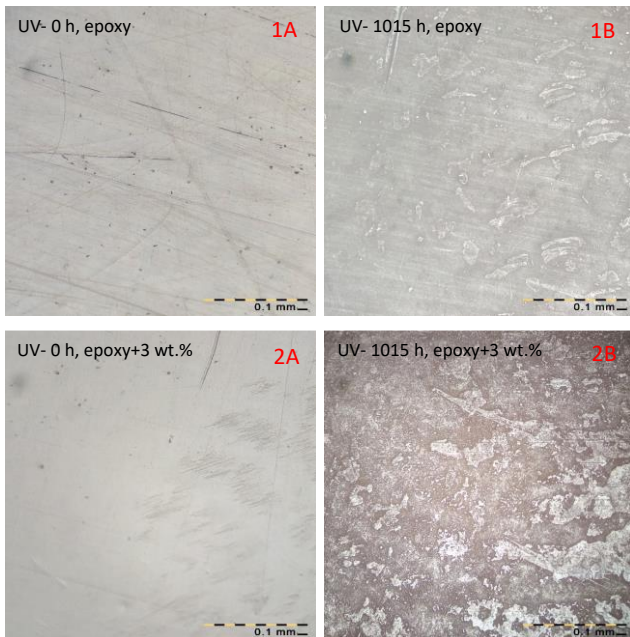
Fig. 16. Neat epoxy sample before (1A) and after UV (1B). Epoxy sample filled with 3 wt.% of thermochromic microcapsules before (2A) and after UV (2B). All under 200× magnification
