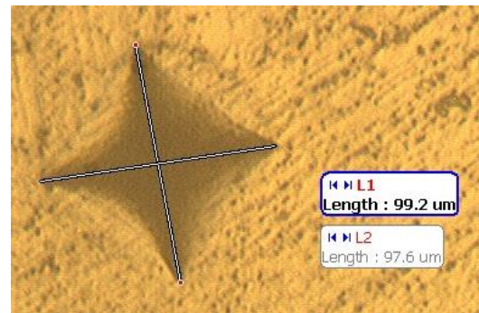
Fig. 7. Elastic image of a neat epoxy sample, the measurement of the diagonal left by the indenter
