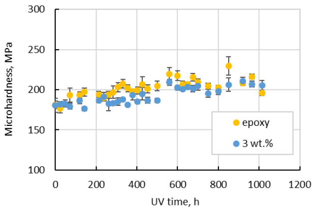
Fig. 14. The microhardness of neat and 3 wt.% filled epoxy samples on UV time
