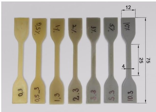
Fig. 1. Dog-bone shape samples with different concentrations of microcapsules
