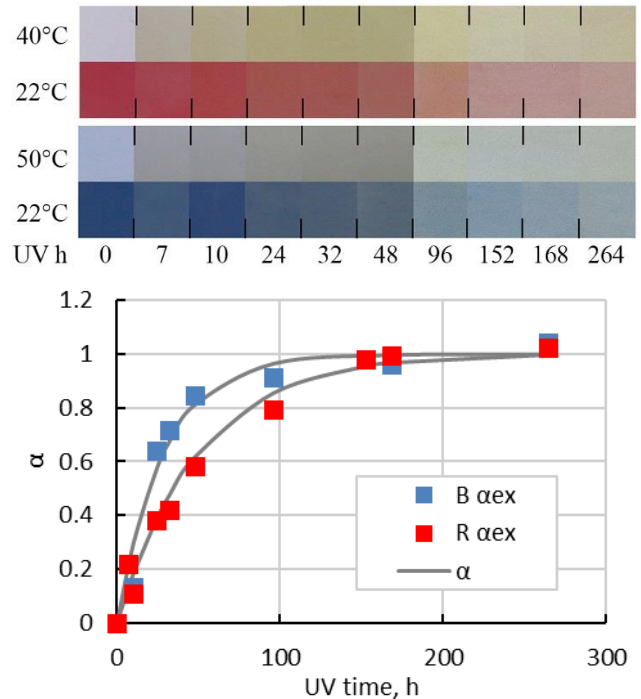
Fig. 13. Samples during UV exposure in colourless and colour phases (top). The kinetics of B and R values change of blue and red colour samples vs UV exposure time, dots are experimental values, solid lines are calculations (bottom). The colour of the experimental dots corresponds to the measured colour
