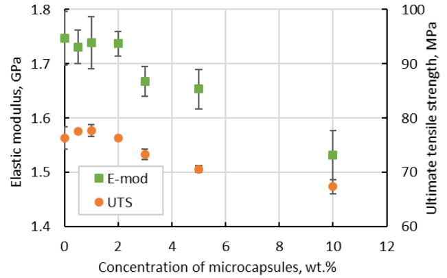
Fig. 6. Elastic modulus (■) and ultimate tensile strength (●) dependence on the concentration of microcapsules in the sample
