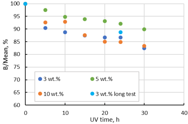
Fig. 11. The change of B/Mean value on UV exposure time for different concentrations of thermochromic microcapsules in the polymer matrix
