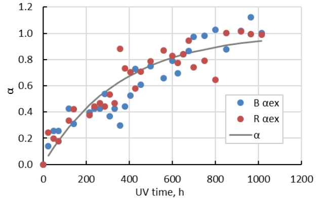
Fig. 12. The kinetics of B (blue dots) and R (red dots) values change in sample vs UV exposure time. Dots for experiment and solid line for calculation [13]
