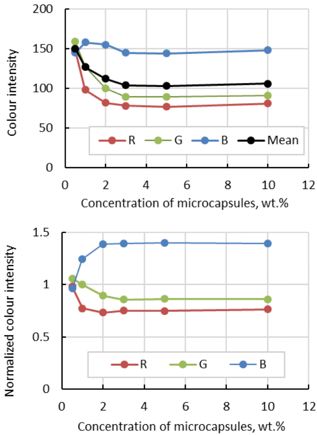
Fig. 5. Colour intensity values of separate channels R, G, B, and Mean dependence on the concentration of microcapsules (top). The dependence of each colour channel R, G, B, normalized to the Mean value on the concentration of microcapsules (bottom) [13]
