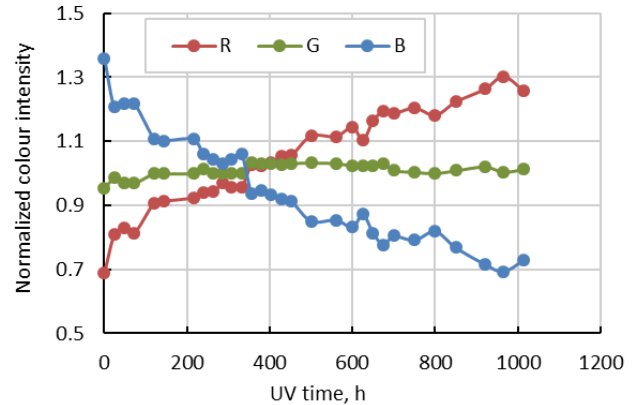
Fig.10. R, G, B channels values normalized to Mean value for filled samples in colour phase during UV exposure [13]
