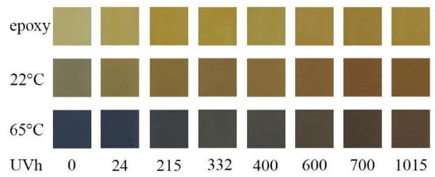
Fig. 9. Samples during UV exposure: neat epoxy (upper line), in colourless (middle line) and colour (lower line) phases
