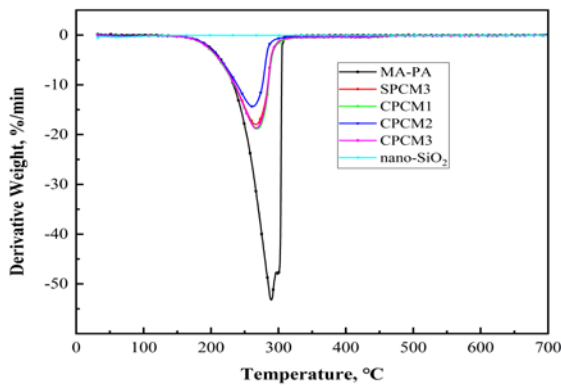
Fig. 7. DTG curves of MA-PA, nano SiO 2 , SPCM3, CPCM1, CPCM2 and CPCM3
