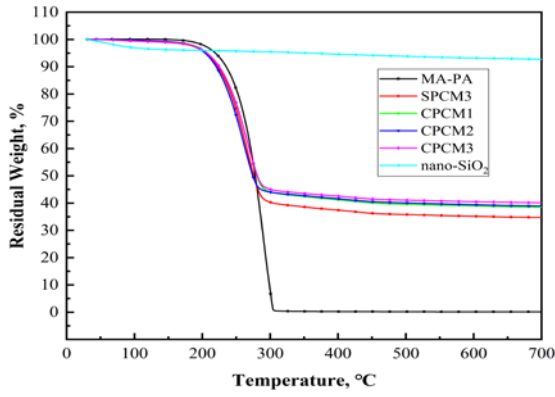
Fig. 6. TGA curves of MA-PA, nano-SiO 2 , SPCM3, CPCM1, CPCM2 and CPCM3
