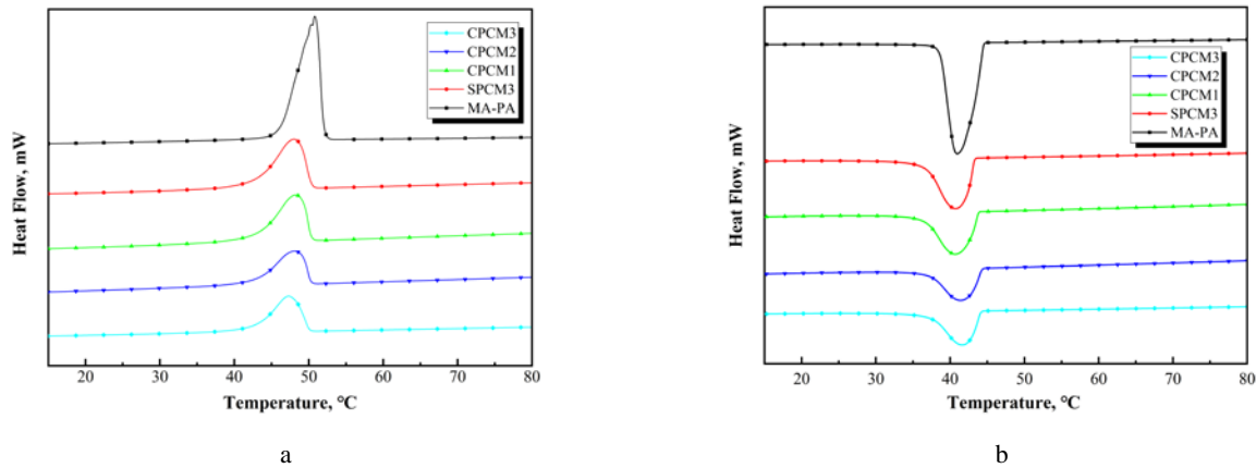
Fig. 5. a – melting DSC curves; b – solidifying DSC curves of MA-PA, SPCM3, CPCM1, CPCM2 and CPCM3
