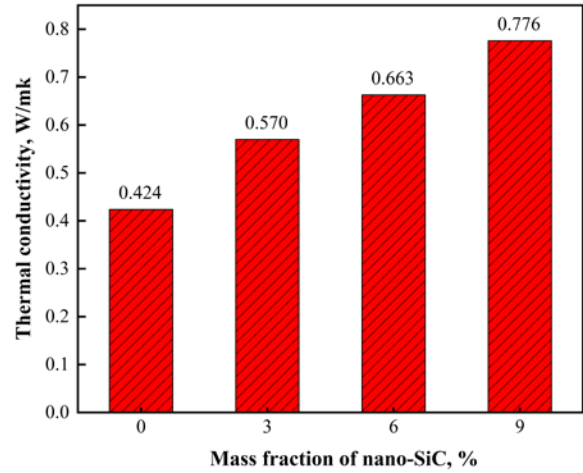
Fig. 8. Thermal conductivity of different composite PCMs
