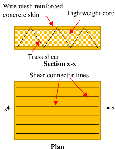
Fig. 1. Concrete sandwich panel
