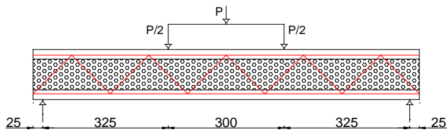
Fig. 4. Test setup for four-point bending
