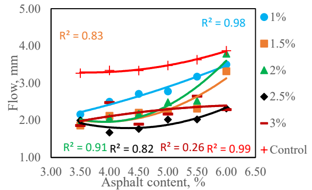
Fig. 7. Relationship between flow and asphalt content
