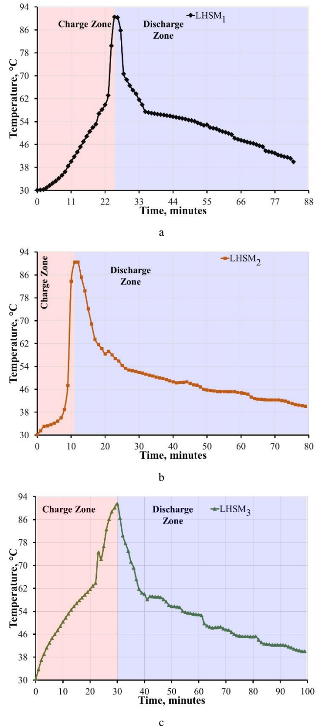
Fig. 3. Charge and discharge behavior for the evaluated samples: a –LHSM 1 ; b –LHSM 2 ; c –LHSM 3
