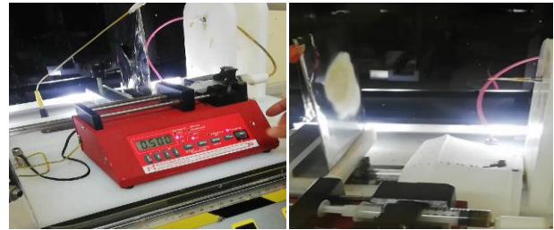
Fig. 1. Electrospinning device and fiber production moment visualization
