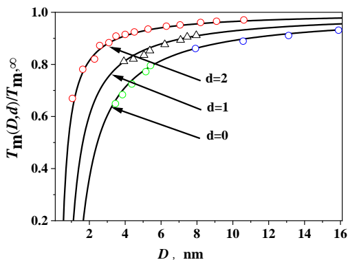
Fig. 1. The function T_m(D, d)/T_m(\infty) of Pb versus D . The solid lines mean the model predictions in terms of Eq. 6 [4, 26, 49, 50]. The symbol \square [26] and \square [49], \circ [4], \triangle [50] are referred to experimental and simulation results for Pb nanoparticles, Pb nanowires, and Pb thin films, respectively
