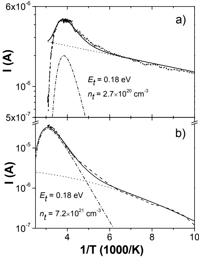
Fig. 4. Experimental curves (dashed curves) and their modelling (solid curves) by taking into account carrier mobility variation (dotted lines) and thermal generation of carriers (dash-dotted curves) in two samples (a and b)
