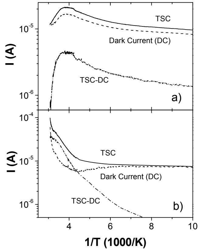
Fig. 3. Experimental TSC spectra of two devices fabricated on the same glass substrate measured after the light excitation (solid curves), dark currents (dashed curves) and their differences (dashed-dotted curves)
