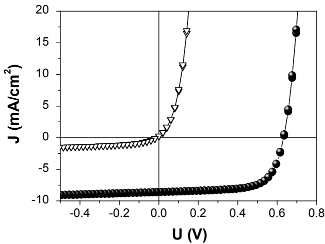
Fig. 2. Current-voltage dependencies in the dark (triangles) and under illumination by AM 1.5 spectrum light with 100 mW/cm 2 power density (dots)
