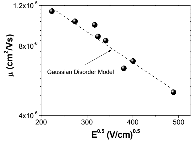
Fig. 5. Mobility dependence versus applied electric field strength and its fitting by the Gaussian Disorder Model.
