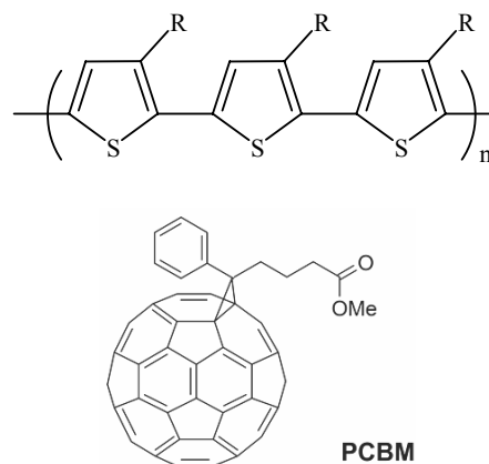
Fig. 1. Structures of the blend constituents P3HT (R = C 6 H 13 ) and PCBM
