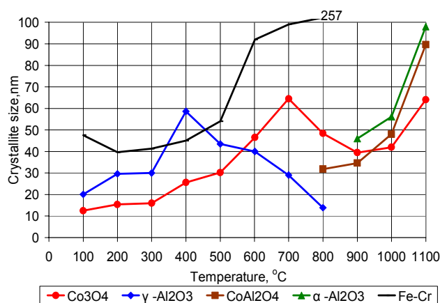
Fig. 6. The distribution of crystallite size of the system „Co-Al-O coating – substrate”
