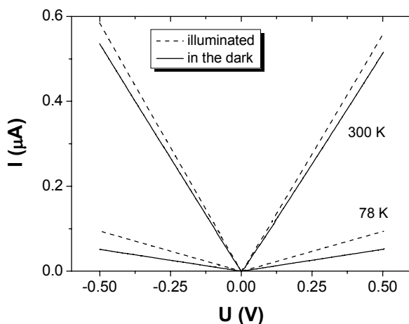
Fig. 2. IV curves of the sample upon illumination by white light (dashed curves) and in the dark (solid lines) at 300 K and 78 K as indicated on the Figure
