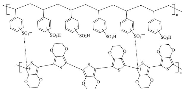
Fig. 1. Chemical structure of PEDT-PSS
