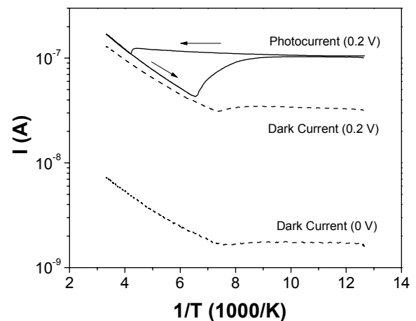
Fig. 7. Temperature dependencies of the photocurrent (PC – solid curves), upon scanning the temperature down and up as indicated by the arrows and the dark current (DC – dashed curves) at 0.2 V bias and without any applied bias
