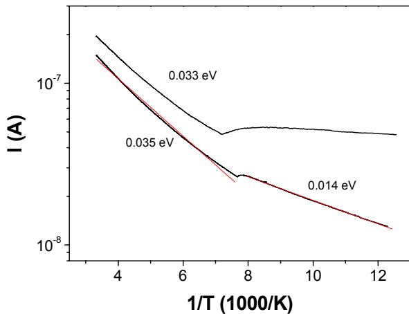
Fig. 5. Dark current temperature dependencies in two samples, measured at 0.5 V applied bias
