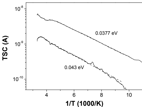
Fig. 6. TSC scans in two samples grown on the same substrate, measured at 0.5 V applied bias after the white light excitation (solid curves). Dashed curves indicate linear fits in Arrhenius scaling
