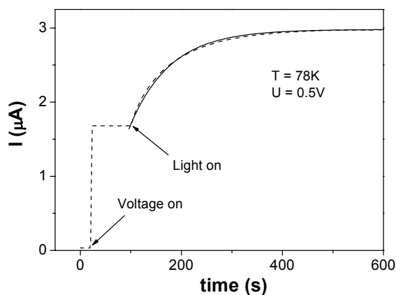
Fig. 3. Sample reaction on applied voltage pulse and white light pulse (dashed curve) as indicated on the Figure. The photocurrent growth could be approximated well by exponential dependence as indicated by the solid curve
