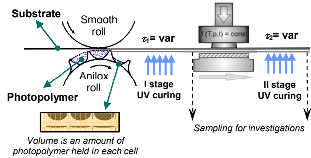
Fig. 2. Schematic view of photopolymer layer formation using two stages of UV curing
