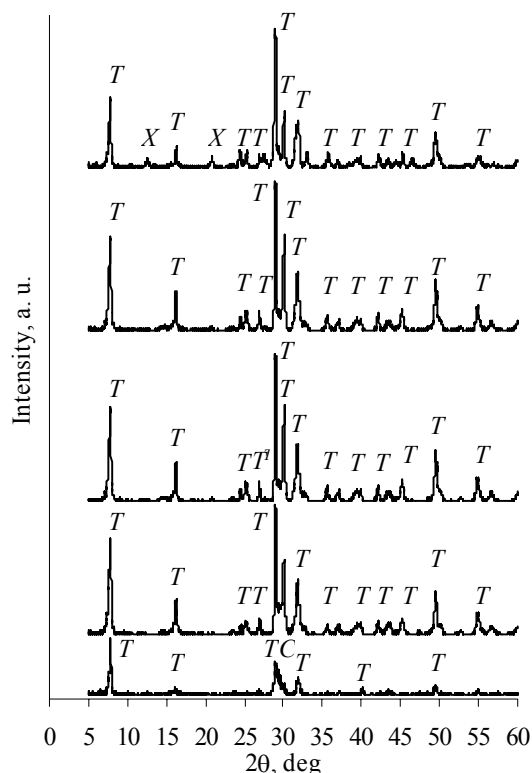
Fig. 7. XRD diffraction patterns of synthesis products at 175 °C temperature, when composition of initial mixtures C/(S+A)=0.083 , amount of additives and synthesis duration: 1 – A/(S+A)=0 , \text{Na}_2\text{O}=0\% , \tau=24 h; 2 – A/(S+A)=0,025 , \text{Na}_2\text{O}=0\% , \tau=24 h; 3 – A/(S+A)=0.025 , \text{Na}_2\text{O}=5\% , \tau=24 h; 4 – A/(S+A)=0.025 , \text{Na}_2\text{O}=0\% , \tau=32 h; 5 – A/(S+A)=0.025 , \text{Na}_2\text{O}=5\% , \tau=32 h. Indexes: T – 1.13 nm tobermorite, C – C-S-H(I), X – xonotlite
