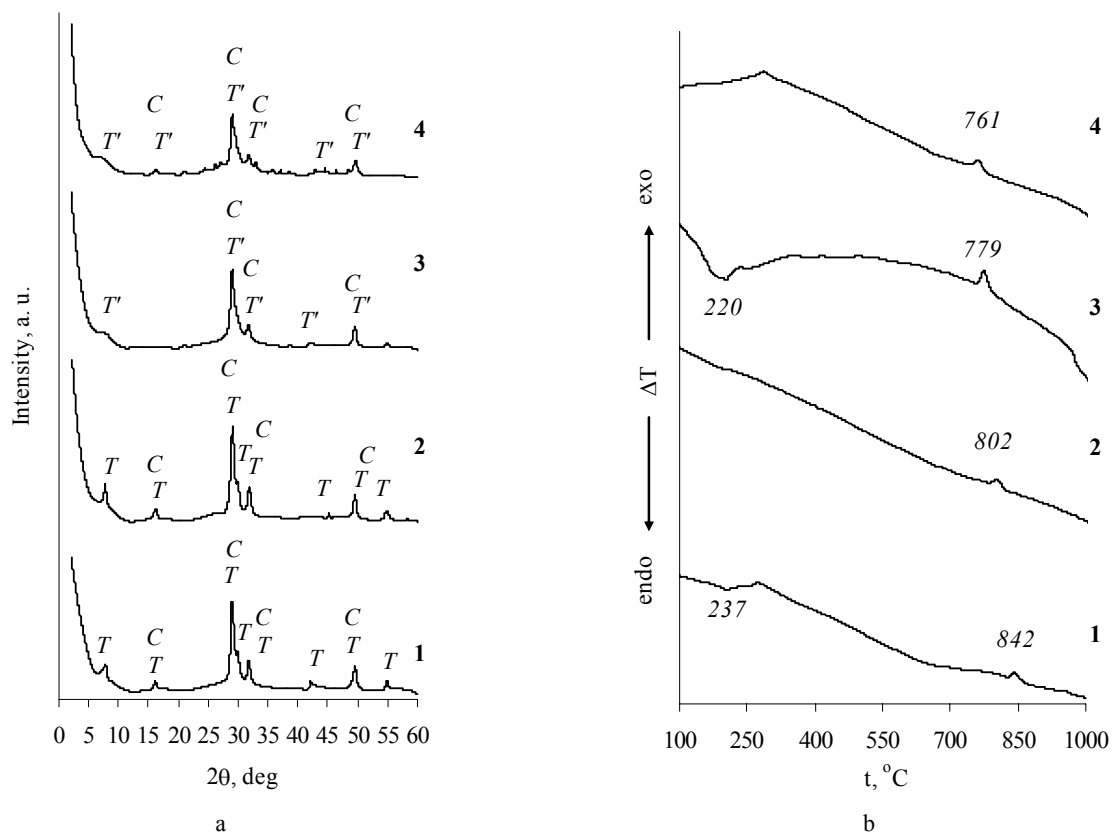
Fig. 2. XRD diffraction patterns and DSC curves of synthesis products from \text{CaO-SiO}_2\text{-nH}_2\text{O} mixtures. Temperature – 175^\circ\text{C} when duration of curing is 16 h and \text{Na}_2\text{O} content, %: 1 – 0; 2 – 5; 3 – 7; 4 – 10. Indexes: C – C-S-H(I), T' – tobermorite gel, T – 1.13 nm tobermorite
