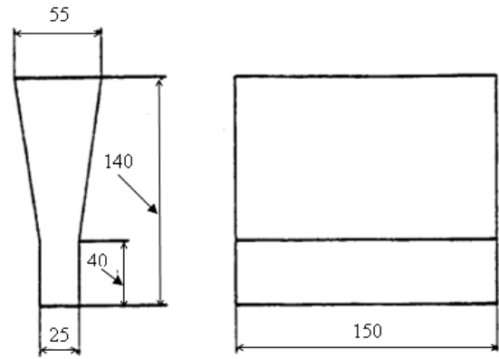
Fig. 1. Geometry of the Y-block ingot (dimensions in mm)
