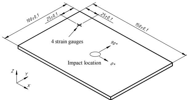
Fig. 1. Laminated composite specimen in accordance with the Airbus Standard (AIITM 1-0010)
