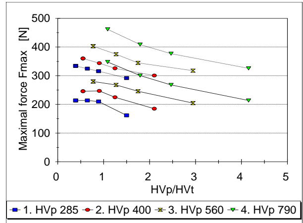
Fig. 1. The maximum normal force component F_{\max} versus the ratio of particle and target material hardnesses HVp and HVt. Dashed lines show Gommel's experimental results [2] and solid lines express our calculations
