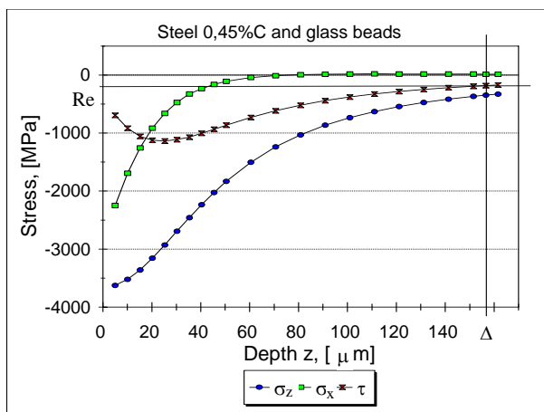
Fig. 3. Shearing stress \tau and principal stresses \sigma_x and \sigma_z under the impact crater of glass particle according. Calculations were made for impact angle 30^\circ and for impact velocity of 13.25 m/s
