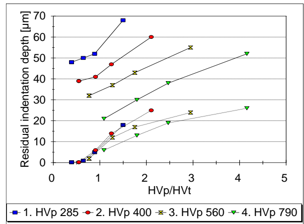
Fig. 2. Residual indentation depth versus the ratio of particle and target material hardness. Dashed lines show the Gommel's experimental results [2] and solid lines express our calculations
