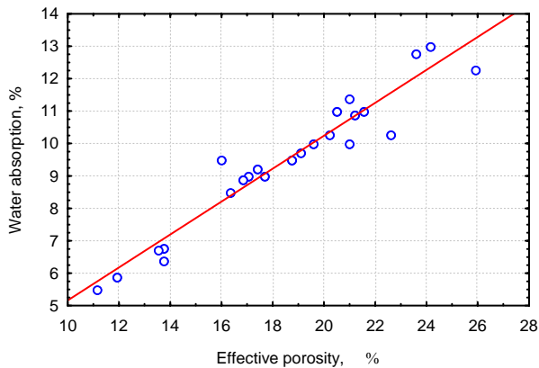
Fig. 1. Ceramic bodies dependence of water absorption on the effective porosity
