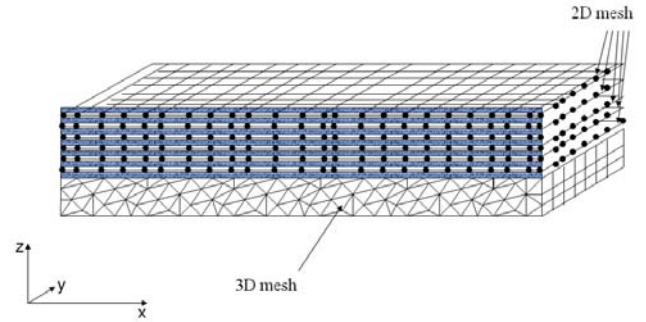
Fig. 4. Finite element mesh
