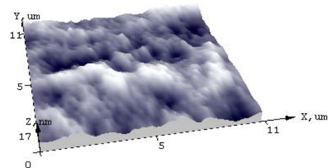
Fig. 7. Atomic force microscope view of the SiO_x doped DLC film surface (average roughness R_a = 2.1 \text{ nm} )
