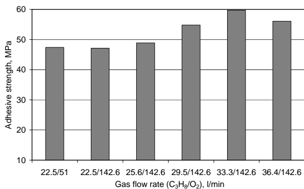
Fig. 7. Dependence of WC-12%Co coating, sprayed by MicroJet gun, adhesive strength on gas flow rate
