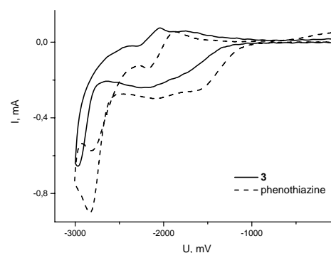
Fig. 2. Cyclic voltammogram: a – of compound 3 and phenothiazine films in ( 0.1\text{ M LiClO}_4 ) acetonitrile solution in three electrode cell.; b – of 3 and phenothiazine in DMF solution (concentrations are 5\text{ mM} ) ( 0.05\text{ M LiClO}_4 ) in two electrode cell. Scan rate was 50\text{ mV/s} , 1st cycle
