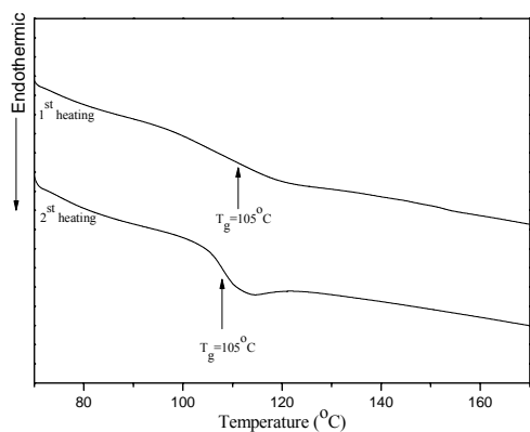
Fig. 1. DSC curve of 3 . Heating rate: 10^\circ\text{C}/\text{min}
