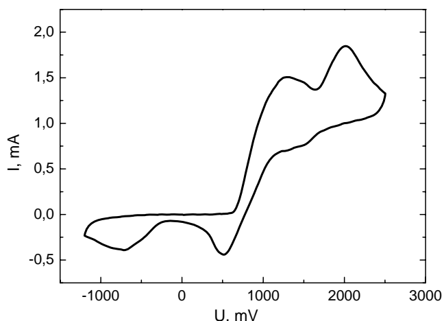
Fig. 2. Cyclic voltammogram of 2 in 0.1 M LiClO 4 acetonitrile solution in three electrode cell. Concentration of 2 is 1 mg/ml. Scan rate: 50 mV/s. 1st cycle. Working electrode – ITO coated glass
