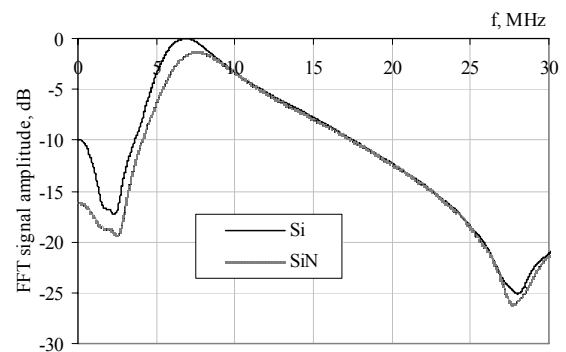
Fig. 12. Calculated dependence echo to the membrane material. CMUT biased 80 % from collapse voltage for circular membrane. d_m = 40 \mu\text{m} , h_g = 0.15 \mu\text{m} , h_i = 0.3 \mu\text{m} , h_e = 0.4 \mu\text{m} , V_{collapse} = 115 \text{ V} for Si membrane and V_{collapse} = 130 \text{ V} , for \text{Si}_3\text{N}_4 membrane V_{pulse} = 40 \text{ V} , t_{pulse} = 60 \text{ ns}
