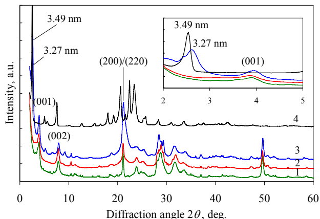
Fig. 2. X-ray diffraction patterns: 1 – synthetic gyrolite, 2 – organically modified pure gyrolite, 3 – organically modified sodium substituted gyrolite, 4 – ODA-Cl
