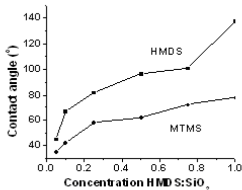
Fig. 6. Contact angles with modifier concentration for coatings after 14 day aging
