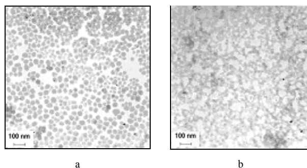
Fig. 1. TEM images of particles obtained from reaction mixtures 3 % \text{SiO}_2 sol and: a – HMDS (0.25), b – MTMS (0.25)
