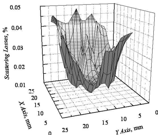
Fig. 10. Light scattering losses map of HMDS modified silica coating on BK-7 glass
