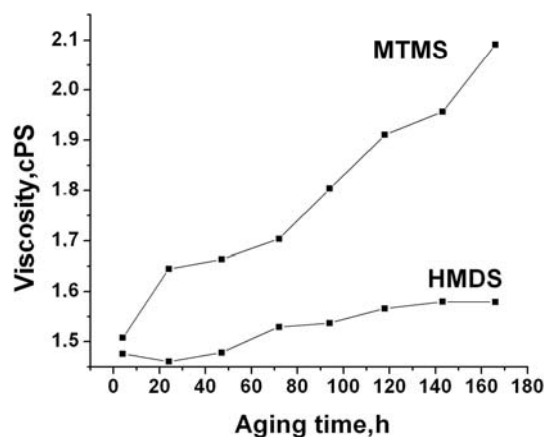
Fig. 2. Variation of viscosity with time of modified sol with MTMS (0.25) and HMDS (0.25) sol
