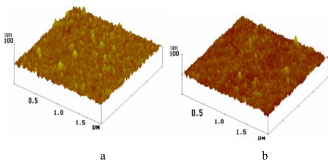
Fig. 4. AFM images of surface morphology of coatings obtained from sol: a – modified HMDS (0.25), b – HMDS (0.1)
