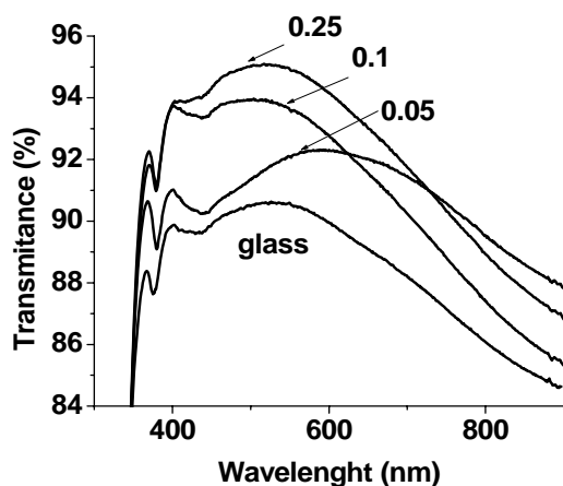
Fig. 9. Transmission spectra for coating on lime glass obtained from modified silica sol with different concentration HMDS
