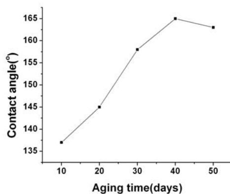
Fig. 7. Variation water contact angles with aging time for HMDS (0.25) modified silica coatings
