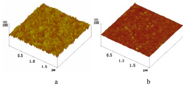
Fig. 3. AFM images of surface morphology of coatings obtained from sol: a – unmodified silica sol, b – MTMS (0.25) modified
