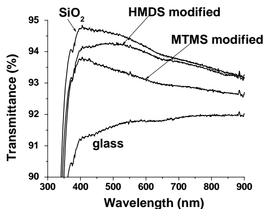
Fig. 8. Transmission spectra for BK-7 glass and coating obtained from sol: a – 3% \text{SiO}_2 , b – modified 0.25 HMDS, c – 0.25 MTMS
