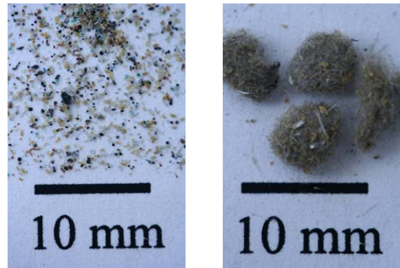
Fig. 8. PCB milled product after 8-time milling in DSL-115: a – separated PCB-powder particles, b – separated glass-fibre
