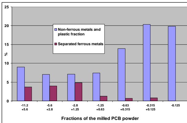
Fig. 7. Results of magnetic separation
