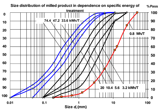
Fig. 3. Dependence of the particle medium size of PCBs on the specific energy of treatment
