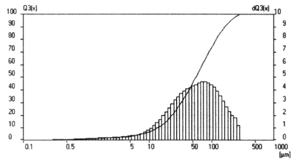
Fig. 4. Laser granulometry of the milled PCB powder
