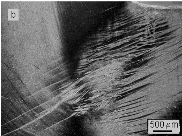
Fig. 3. Band morphology revealed in SC Nb by longitudinal sections (TD plane) in shear region of diametric (a) and 0.5 radius (b) sections at ECAP. The GB forming initiation is shown in (a) by arrows
