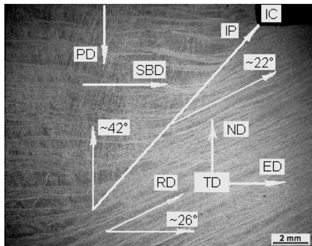
Fig. 2. Schematic drawing of ECAP in a shear region (near intrinsic corner (IC) of ECAP die) during next passes by B_c route is shown. The pressure direction are shown by arrows (PD), normal direction (ND), extrusion direction (ED), transverse direction (TD), shear bands direction (SBD) before intersection plane (IP) and ribbons direction (RD) after IP in SPD Nb. The angles between these directions are: 42° – between PD and IP, 22° – between IP and RD, 26° – between RD and ED
