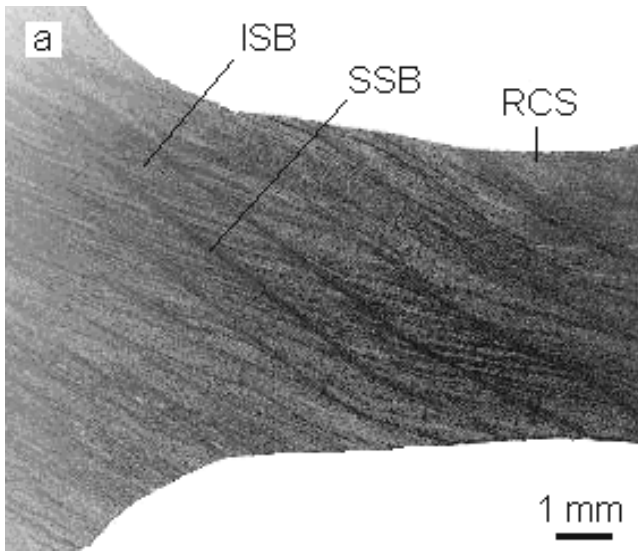
Fig. 6. The double-banded microstructure of pure Nb after SPD under ECAP and followed HCV deformation. Designations: ISB – initial shear bands, SSB – secondary shear bands, RCS – reduced cross section
