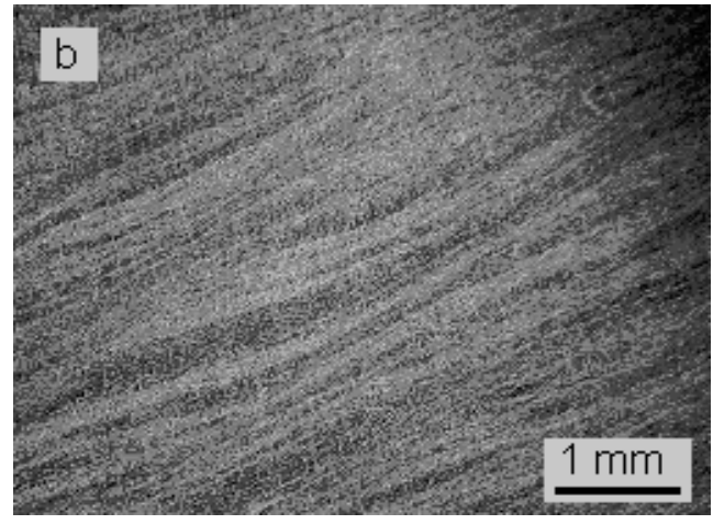
Fig. 4. The optical images of shear band's structure after three B_c passes of ECAP nearby shear zone (a) and in pressed Nb sample (b)
