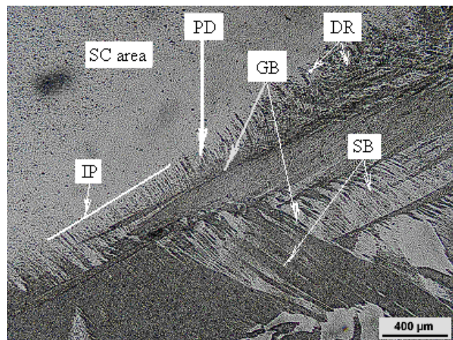
Fig. 1. Optical image of specimen (Nb) in a shear region of ECAP after first pass is shown. Designations: SC – single crystal area, PD – pressure direction, IP – intersection plane, GB – grain boundary, DR – dislocation ribbons, SB – shear bands
