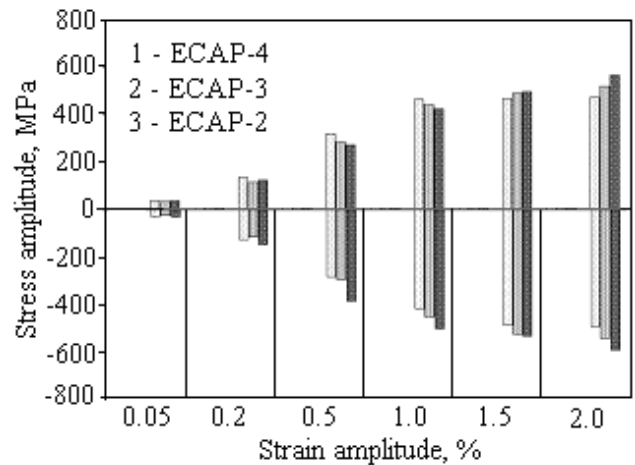
Fig. 5. The strain- and stress amplitudes diagram of samples for first cycle under HCV deformation. Designations: 1 – 4 passes of ECAP, 2 – 3 passes and 3 – 2 passes
