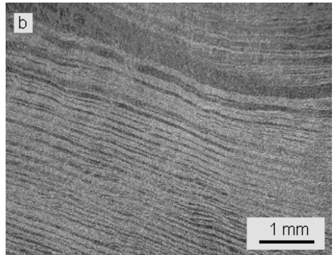
Fig. 6. The double-banded microstructure of pure Nb after SPD under ECAP and followed HCV deformation. Designations: ISB – initial shear bands, SSB – secondary shear bands, RCS – reduced cross section
