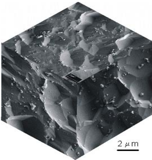
Fig. 8. The FE SEM 3D picture of pure Nb after four passes by B_c route of ECAP
