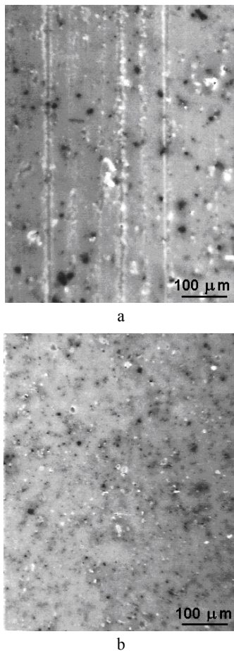
Fig. 4. Surface of the unmodified acrylic coating (a) and the one modified with copper nanoparticles (b) after scratch test with the use of 800 A abrasive paper (containing silicon carbide grains)
