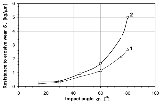
Fig. 2. Resistance to erosive wear of acrylic coatings modified with copper nanoparticles (1 – acrylic coating, 2 – acrylic coating containing 3.5 % copper nanoparticles by weight)
