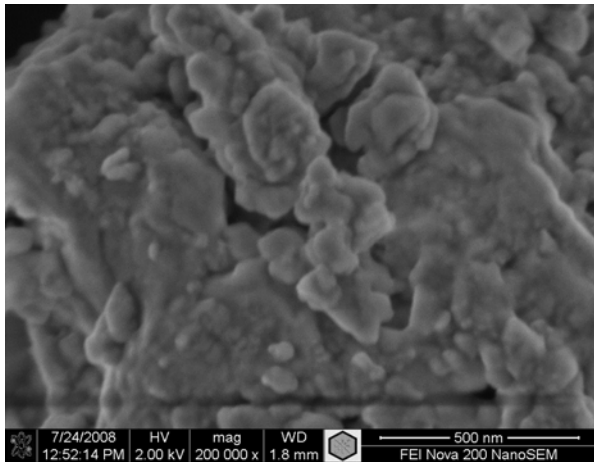
Fig. 1. Morphology of copper nanoparticles
