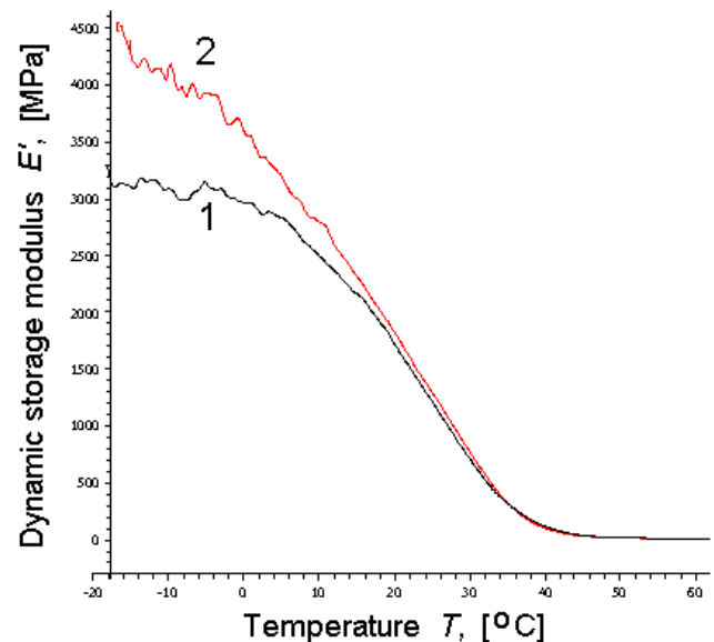
Fig. 5. Dynamic storage modulus E' of acrylic coatings (1) and acrylic coatings modified with copper nanoparticles (2)
