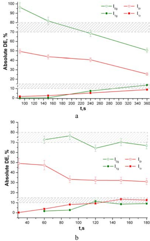
Fig. 2. Diffraction efficiency dependence on the duration of PCE treatment in CF 4 /O 2 plasma: a) CF 4 /O 2 – 85 % / 15 %, t = 90 s – 360 s, b) CF 4 /O 2 – 80 % / 20 %, t = 30 s – 180 s. “I 1 ” and “I 0 ” stands for the diffraction orders (average of I_{\pm 1} and I_0 respectively) and “g”, “r” indicates the used wavelength (532 nm and 632.8 nm respectively). Dashed region indicates limits of the necessary diffraction efficiency
