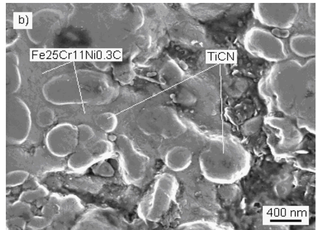
Fig. 4. Wear surface of composite under dry sliding with phase's indication (a) and stainless steel binder with in situ TiCN particles (b)
