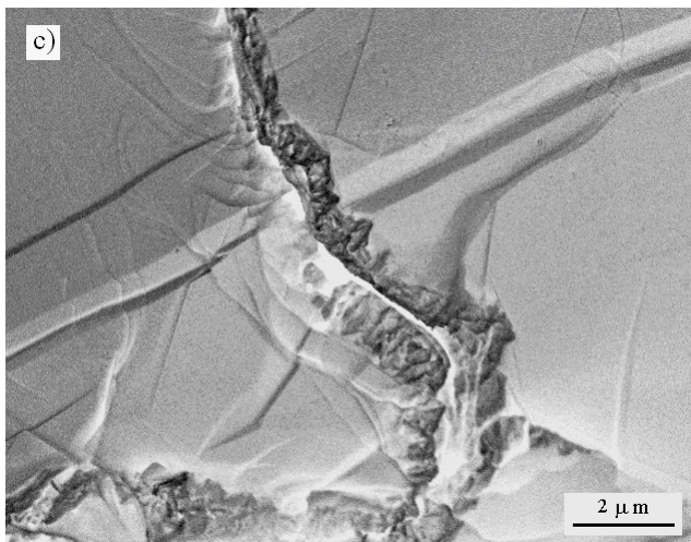
Fig. 5. The fractures are of boron carbide based composite (a), by atomic layers of boron carbide crystallite (b) and crystal fracture in cross-section to crystal (c)
