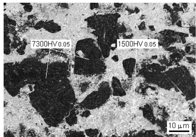
Fig. 1. SHS processed raft c-BN-based composite with microhardness indication
