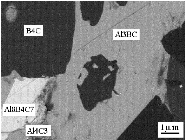
Fig. 3. The mechanism boron aluminum carbide (Al 3 BC) forming in composite binder phase during SHS reaction is presented
