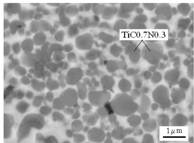
Fig. 2. Microstructure of binder phase with indication of ultrafine precipitated of stoichiometry titanium carbonitrides
