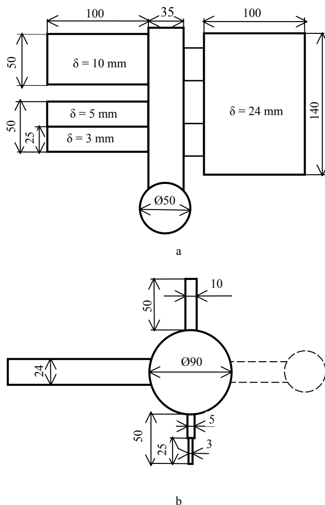
Fig. 1. Horizontal (a) and vertical (b) test castings (dimensions in millimetres)
