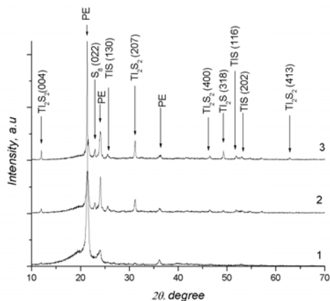
Fig. 9. X-ray diffraction patterns of thallium sulphide layers on the surface of PE. PE initially treated with a solution of H 2 S 33 O 6 at 80 °C for different times and then immersed in Tl 2 SO 4 solution at 80 °C for 10 min. Sulphurisation time (min): 1–15, 2–60, 3–120
