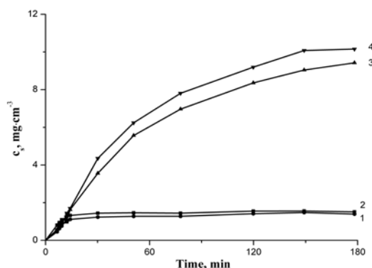
Fig. 2. Dependence of the content of sulphur in layer on PE film on sulphurization time under treatment it with solutions of H_2S_{33}O_6 . The temperature ( ^\circ C ) of H_2S_{33}O_6 solution: 1–25, 2–40, 3–60, 4–80
