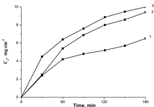
Fig. 1. Dependence of the content of sulphur in layer on PE film on sulphurization time under treatment it with solutions of H_2S_nO_6 at 60^\circ C . The average number of sulphur number atoms ( n ) in polythionic acid molecule: 1–21; 2–33; 3–45
