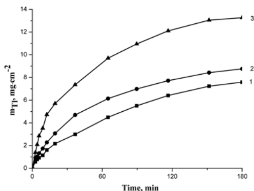
Fig. 6. Dependence of thallium content in sulphide layer on PE film on sulphurisation time under treatment it with solution of H_2S_{33}O_6 at 80 °C for different periods of time. The period of treatment with 0.1 M Tl_2SO_4 solution at 80 °C was 10 min. The concentration ( mol \cdot dm^{-3} ) of Tl_2SO_4 solution: 1–0.001, 2–0.05, 3–0.1
