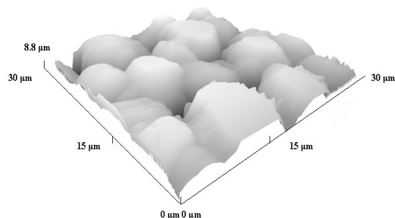
Fig. 11. AFM image of Tl x S y films on polyethylene. PE initially treated with a solution of H 2 S 33 O 6 at 60 °C for 120 min and then immersed in Tl 2 SO 4 solution at 80 °C for 10 min
