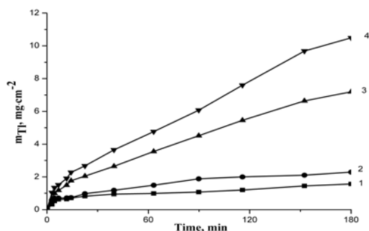
Fig. 7. Dependence of thallium content in sulphide layer on PE film on sulphurization time under treatment it with solution of H_2S_{33}O_6 at 60 °C for different periods of time. The sulphured PE treated with 0.1 M Tl_2SO_4 solution at 80 °C. Duration (min) of sulphured PE treatment with Tl_2SO_4 solution: 1–2, 2–5, 3–10, 4–20
