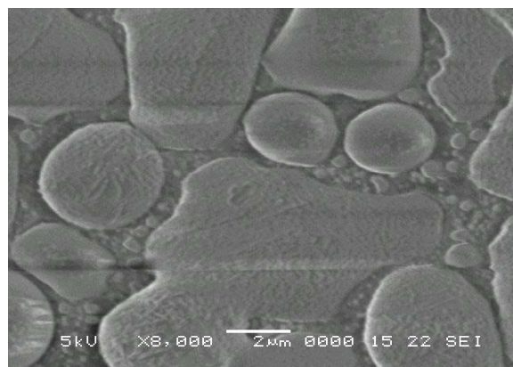
Fig. 10. SEM image of Tl x S y films on polyethylene. Image area (16×10) μm 2
