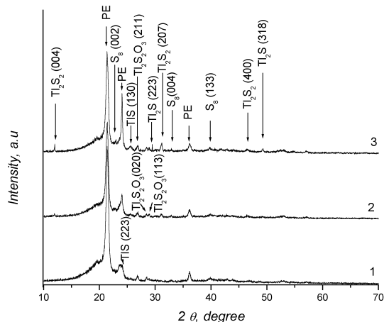
Fig. 8. X-ray diffraction patterns of thallium sulphide layers on the surface of PE. PE initially treated with a solution of H_2S_{33}O_6 at 60 °C for different times and then immersed in Tl_2SO_4 solution at 80 °C for 10 min. Sulphurization time (min): 1–15, 2–60, 3–120
