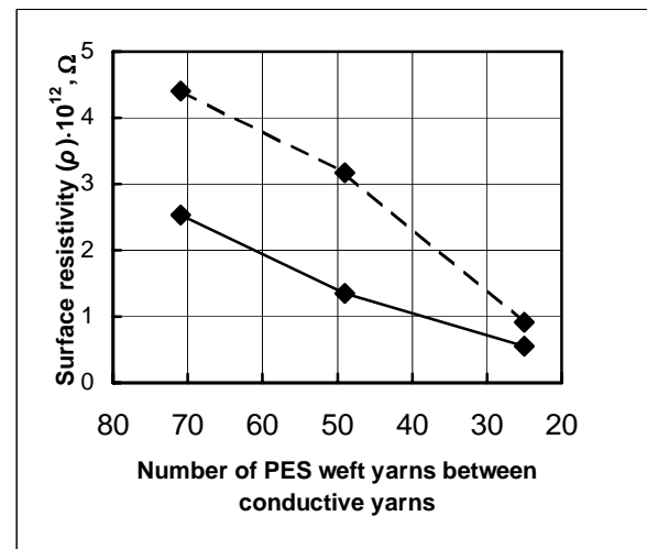
Fig. 3. Surface resistivity of the fabrics versus number of PES weft yarns between the conductive yarns (— as received; - - - after 5 washing cycles) (Control fabric: as received \rho = 9.43 \times 10^{12} \Omega ; after 5 wash. cycles \rho = 9.98 \times 10^{13} \Omega )
