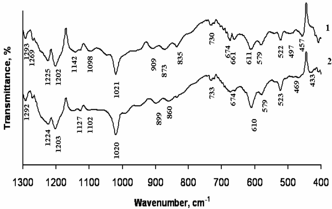
Fig. 1. IR absorption spectra of a PA films treated with 0.004 \text{ mol}\cdot\text{dm}^{-3} solution of H_2S_{12}O_6 at 10 \text{ }^\circ\text{C} different time. Sulfuration time, h: 1 – 2, 2 – 6
