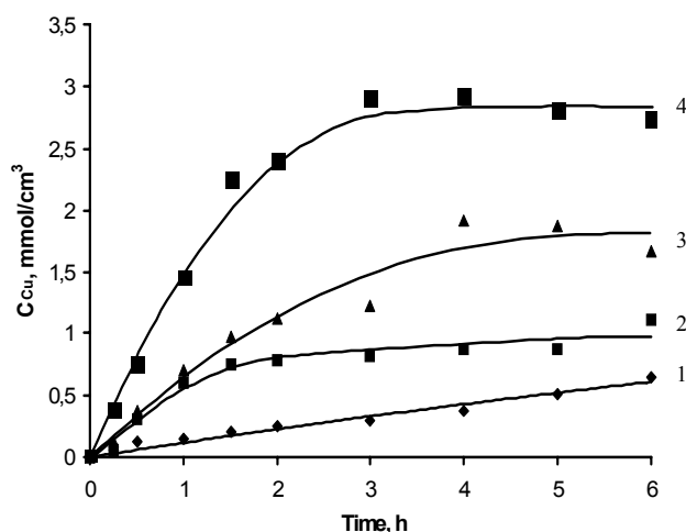
Fig. 7. Dependence of the concentration of copper in sulfide layer on PA film on sulfurization time when treating it with 0.004 \text{ mol}\cdot\text{dm}^{-3} solution of \text{H}_2\text{S}_{12}\text{O}_6 at different temperatures. The temperature ( ^\circ\text{C} ) of \text{H}_2\text{S}_{12}\text{O}_6 solution: 1 – 10, 2 – 20, 3 – 30, 4 – 40
