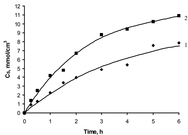
Fig. 6. Change of sulfur concentration in PA with time during its treatment with the solution of \text{H}_2\text{S}_{12}\text{O}_6 of different concentration at the temperature of 40^\circ\text{C} . Concentration, \text{mol}\cdot\text{dm}^{-3} : 1 – 0.002, 2 – 0.004
