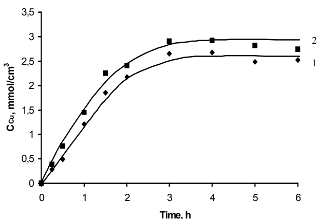
Fig. 8. Dependence of the concentration of copper in sulfide layer on PA film on sulfurization time when treating it with solution of \text{H}_2\text{S}_{12}\text{O}_6 of different concentration at the temperature of 40^\circ\text{C} . Concentration, \text{mol}\cdot\text{dm}^{-3} : 1 – 0.002, 2 – 0.004
