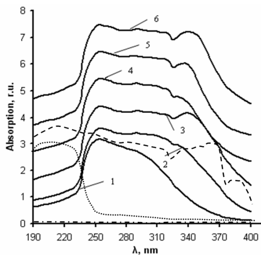
Fig. 3. UV absorption spectra of PA films (..... – without compensation, - - - - using PA absorption compensation), PA films treated with 0.004 \text{ mol}\cdot\text{dm}^{-3} solution of \text{H}_2\text{S}_{12}\text{O}_6 at 20^\circ\text{C} different time and of the 0.004 \text{ mol}\cdot\text{dm}^{-3} solution of \text{H}_2\text{S}_{12}\text{O}_6 - - - - - Sulfurization time, h: 1 – 0.25, 2 – 0.5, 3 – 1.5, 4 – 3.0, 5 – 4.0, 6 – 5.0
