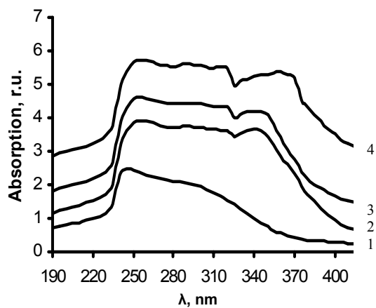
Fig. 4. UV absorption spectra of PA films treated 1.5 h with 0.004 \text{ mol}\cdot\text{dm}^{-3} solution of \text{H}_2\text{S}_{12}\text{O}_6 at different temperature. Sulfurization temperature, ^\circ\text{C} : 1 – 10, 2 – 20, 3 – 30, 4 – 40
