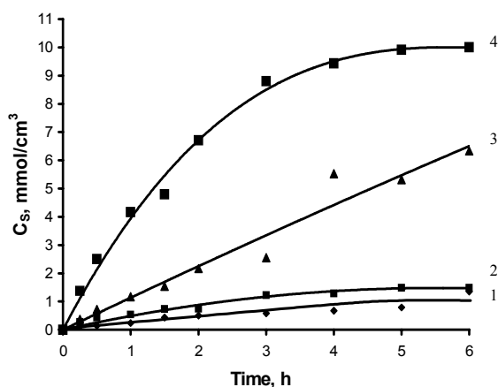
Fig. 5. Change of sulfur concentration in PA with time during its treatment with 0.004 \text{ mol}\cdot\text{dm}^{-3} solution of \text{H}_2\text{S}_{12}\text{O}_6 at different temperatures. The temperature ( ^\circ\text{C} ) of \text{H}_2\text{S}_{12}\text{O}_6 solution: 1 – 10, 2 – 20, 3 – 30, 4 – 40
