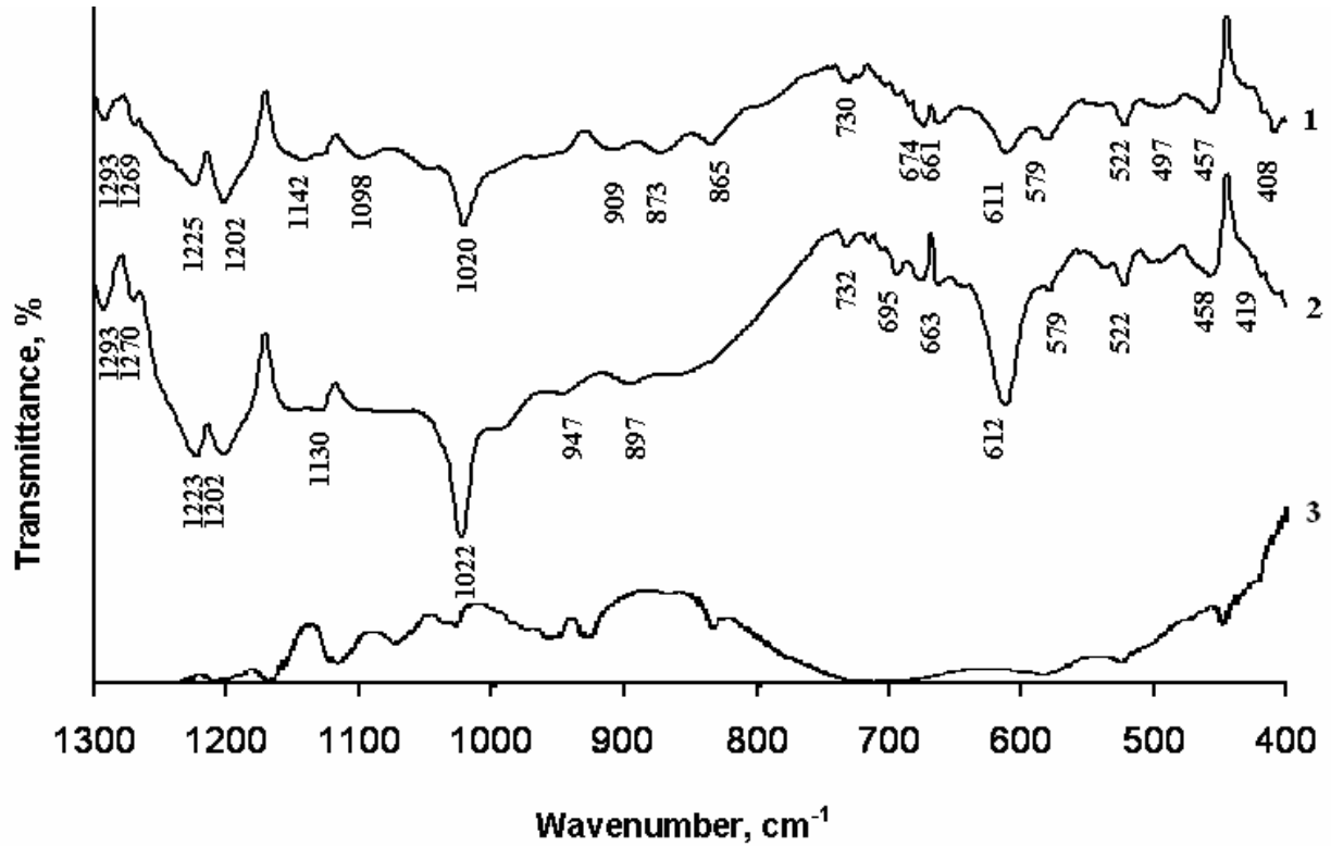
Fig. 2. IR absorption spectra of a PA films treated during 2 h with 0.004 \text{ mol}\cdot\text{dm}^{-3} solution of H_2S_{12}O_6 (1, 2) and of initial untreated PA (3). PA treatment with H_2S_{12}O_6 temperature, ^\circ\text{C} : 1 – 10, 2 – 20
