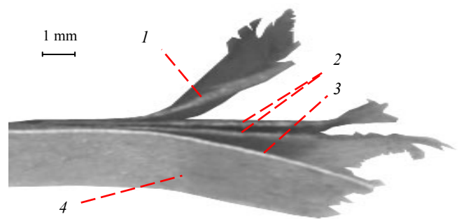
Fig. 9. Photo of flocked sample made from 0.5 mm-length Capron flock and paperboard Duoplex UD-3, when testing the number of double-folds: 1 – bottom layer of the paperboard; 2 – insert; 3 – top layer; 4 – flock coating
