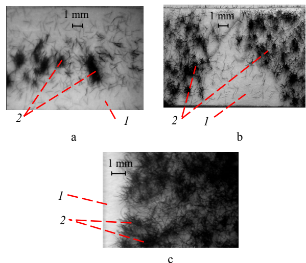
Fig. 6. Photo of glued (glue Eukalin) flocked samples (view from above) made from 1 mm-length Capron flock on paperboard Arktika GC-1 after breaking off: 1 – paperboard; 2 – broken off flock fibers
