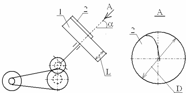
Fig. 1. Laboratory pan granulator: 1 - granulators pan; 2 - reciprocating scraper
