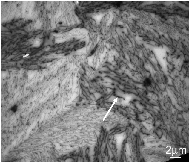
Fig. 7. The carbide situated on the bainitic ferrite/austenite interface (see the arrow), \tau_i = 540 min, the two-stage collodion-carbon replica, TEM
