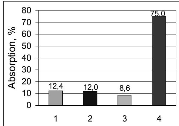
Fig. 6. The water absorption of silicate products (after soaking in water for 48 h): 1 – silicate block; 2, 3 – split face brick: 2 – with hydrophobized facade surface; 3 – with fully hydrophobized surface; 4 – AAC [25]
