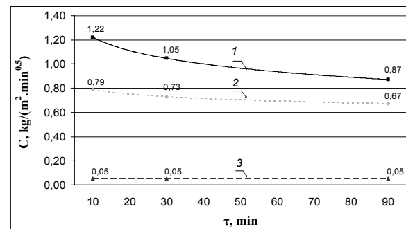
Fig. 3. The impact of time of impregnation on coefficient of water adsorption due to capillary action in the silicate samples: 1 – silicate block ( \rho = 1740 kg/m 3 ); 2, 3 – split face brick, \rho = 1870 kg/m 3 : 2 – not hydrophobized, 3 – hydrophobized
