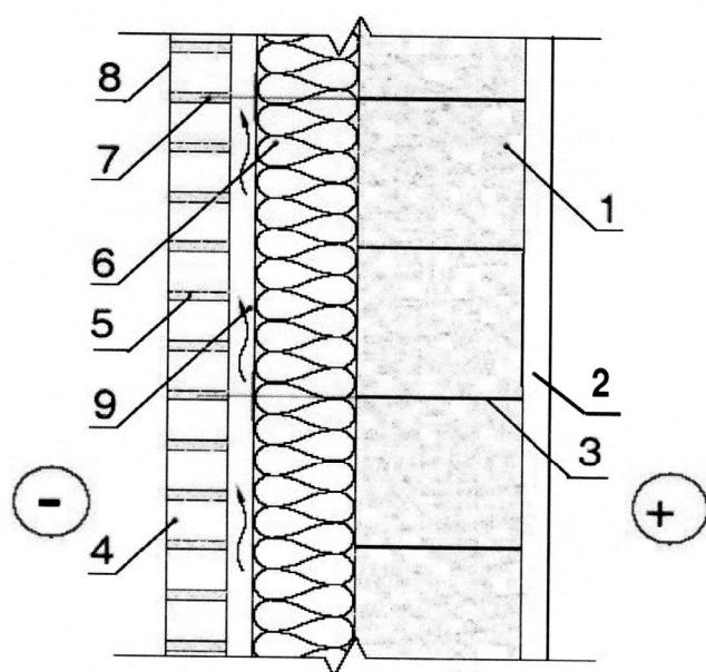
Fig. 1. Multilayer enclosure of silicate elements: 1 – silicate block; 2 – plaster; 3 – adhesive; 4 – split face brick; 5 – hydrophobic masonry mortar; 6 – layer of thermo-insulating material; 7 – flexible bonds; 8 – hydrophobic surface; 9 – air gap [1]
