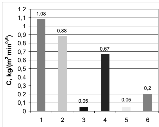
Fig. 4. The values of capillary water adsorption coefficient in silicate masonry products of enclosure after soaking for 90 min: 1 – plaster; 2 – silicate block; 3 – adhesive; 4 – not hydrophobized split face brick; 5 – hydrophobized face brick; 6 – mortar
