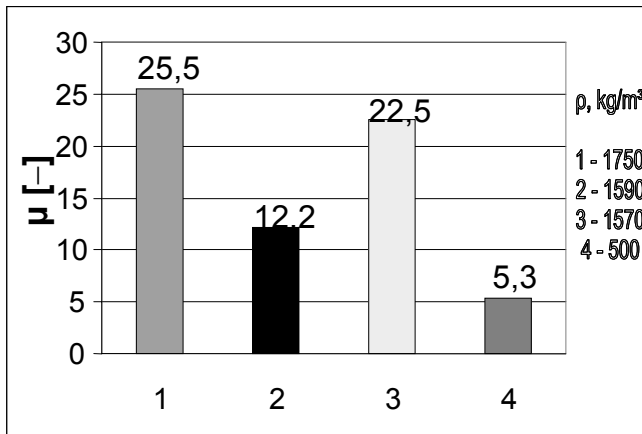
Fig. 5. The values of water vapour diffusion coefficient of silicate samples: 1 – silicate block; 2 – plaster; 3 – adhesive; 4 – AAC [18]
