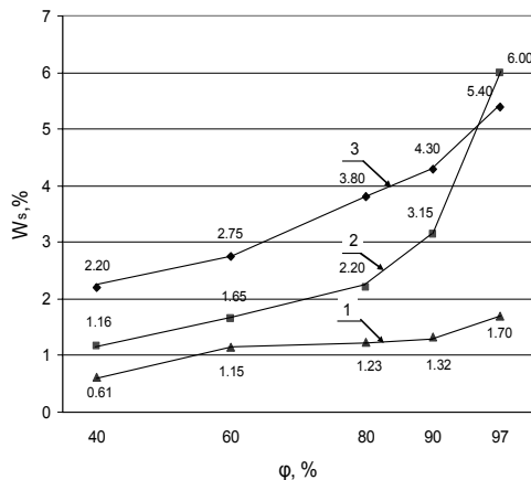
Fig. 2. The influence of relative air humidity ( \phi ) on silicate products sorption ( w_s ): 1 – brick's sample with hydrophobic surface; 2 – not hydrophobic brick's sample; 3 – AAC [18]
