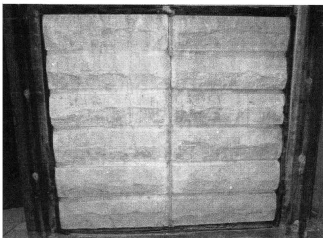
Fig. 8. The wall fragment out of silicate split face bricks
