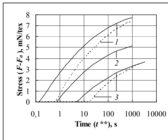
Fig. 6. Inverse relaxation (IR) in PES yarn over time t^{**} after the blockage of recovery (VR) at different strains \epsilon'_a : primary extension \epsilon_i = 10.0\% ; sustention times \theta_i = 100 s (—), and \theta_i = 1000 s (- - -); strains \epsilon'_a , %: 1 – 1.00; 2 – 0.60; 3 – 0.30
