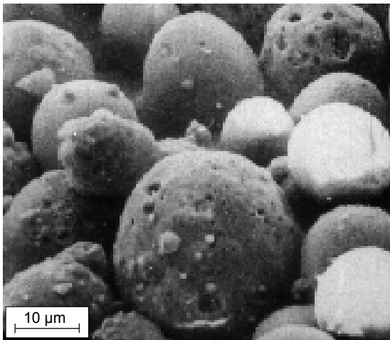
Fig. 2. Morphology of glass microspheres
