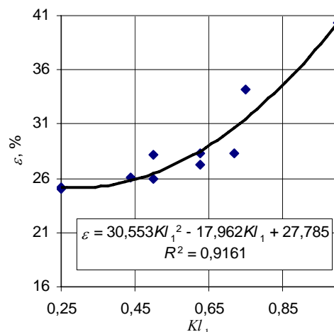
Fig. 4. The dependence of \varepsilon elongation at break on the weave factor Kl_1 having deduced the warp and weft rib weaves
