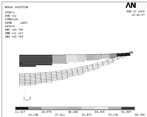
Fig. 5. Displacement pattern for steel leaf spring
