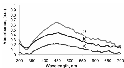
Fig. 1. The UV-VIS spectra of Ag colloid. Time after synthesis: a – 1 hour, b – 2 weeks, c – 3 weeks
