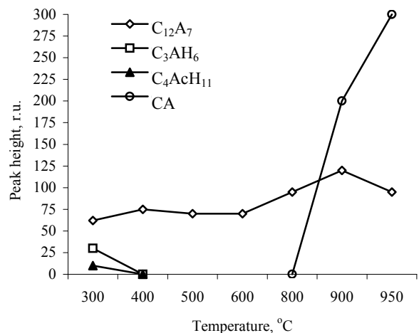
Fig. 3. Changes of peak height of minerals ( C_3AH_6 ( d = 0.229 nm), C_{12}A_7 ( d = 0.220 nm), C_4AcH_{11} ( d = 0.76 nm) and CA ( d = 0.297 nm)) representative peak after firing
